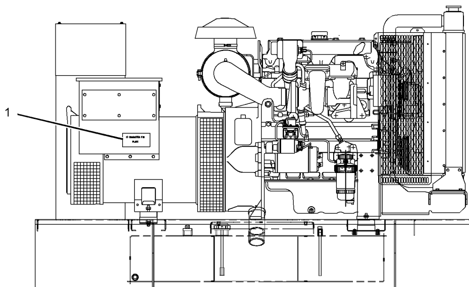
PEP 1000 SERIES (RIGHT SIDE VIEW)
