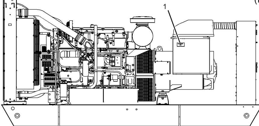
CAT 3456 / 3406 / C18 (COMMON GENSET) (LEFT SIDE VIEW)
